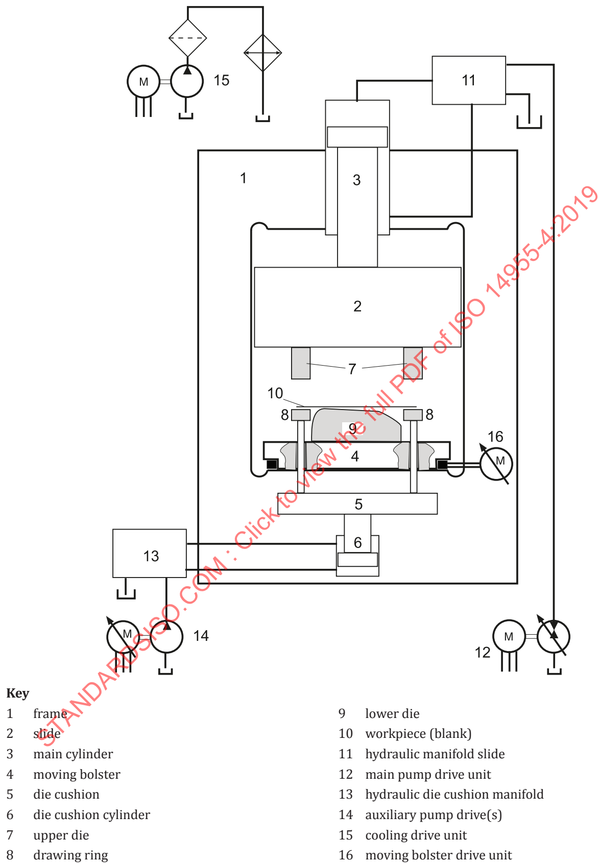
Figure A.1 — Example of a hydraulic double action press
