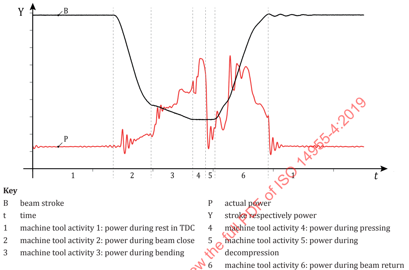
Figure C.3 — Example of beam power during a cycle of a hydraulic press brake
