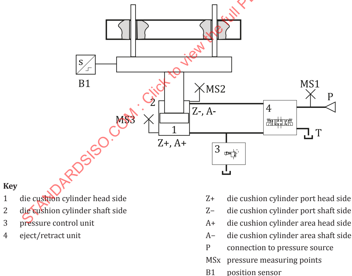
Figure A.5 — Example of a die cushion hydraulic without energy recovery
