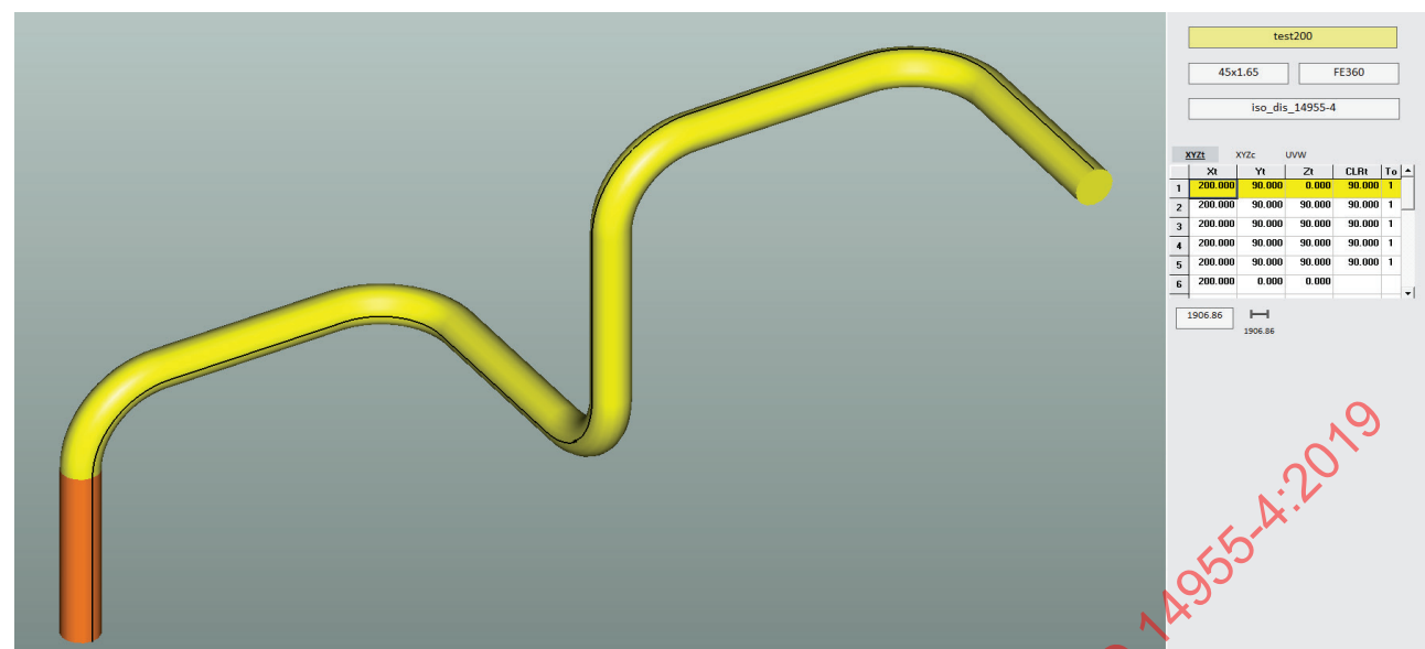
Figure 11 — Test workpiece with 90° bend every 200 mm
