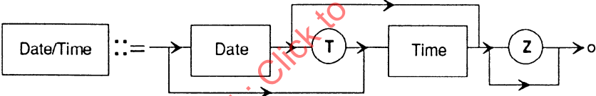
Figure 2-10 Date/Time Syntax Diagram
