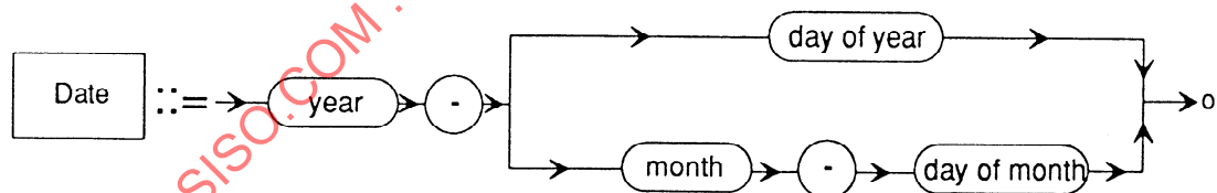
Figure 2-8 Date Syntax Diagram
