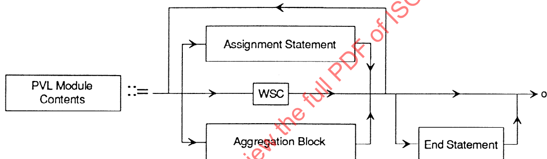
Figure 2-1 PVL Module Contents Syntax Diagram
