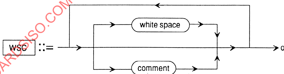
Figure 2-2 White Space/Comment Syntax Diagram
