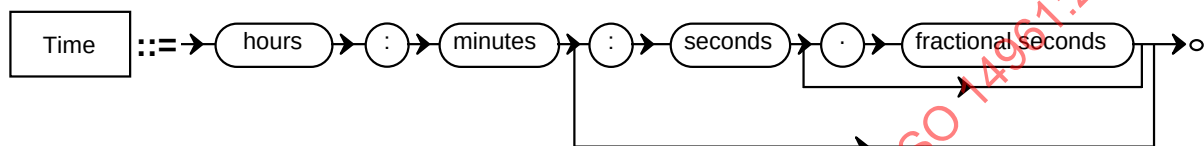
Figure 2-9: Time Syntax Diagram
