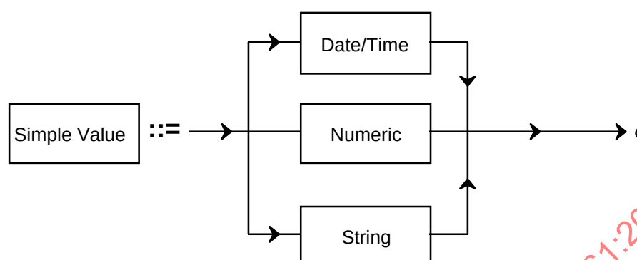
Figure 2-6: Simple Value Syntax Diagram
