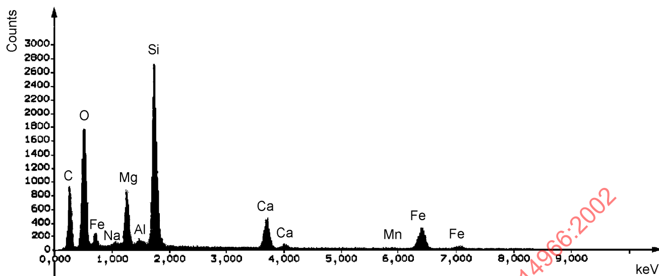
e) Fibre of reference actinolite (no gold coating)
