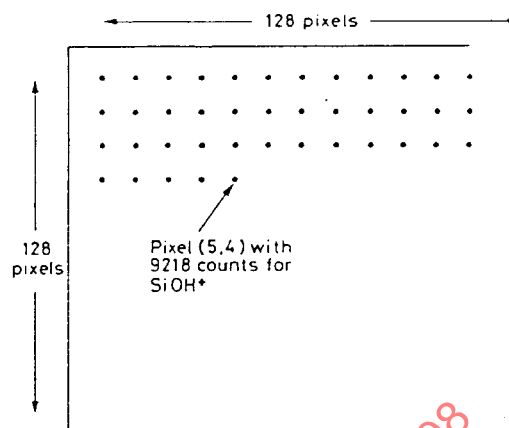
Figure A.2 - A SIMS map of one element setting the mass spectrometer to 45 amu. This illustrates the first block of the example in B.2.3.
