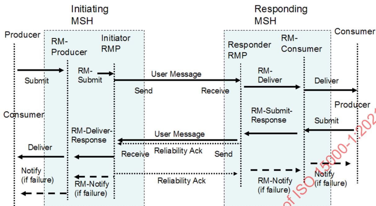
Figure 14: Reliable Two-Way/Sync MEP
