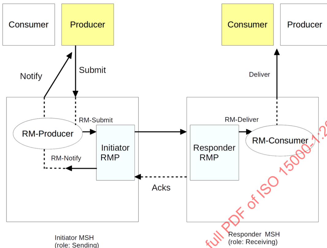
Figure 10: Sending an ebMS Message Reliably
