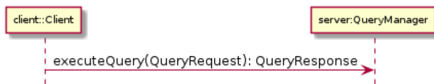
Figure 12 Query protocol
