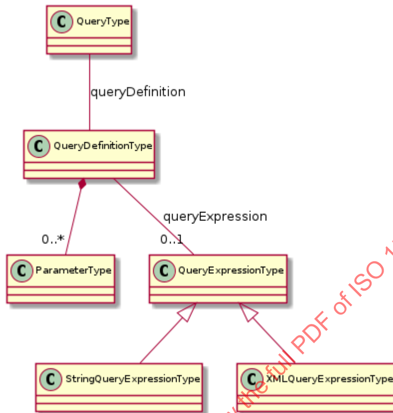
Figure 8 query information model
