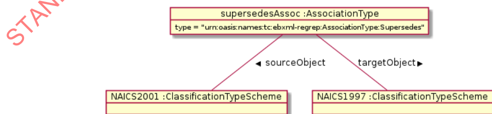
Figure 3 association example
