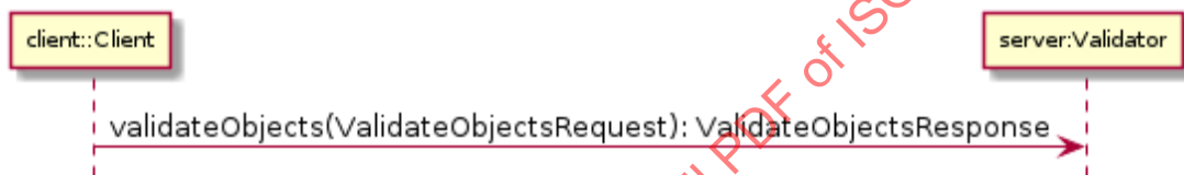
Figure 17 ValidateObjects protocol
