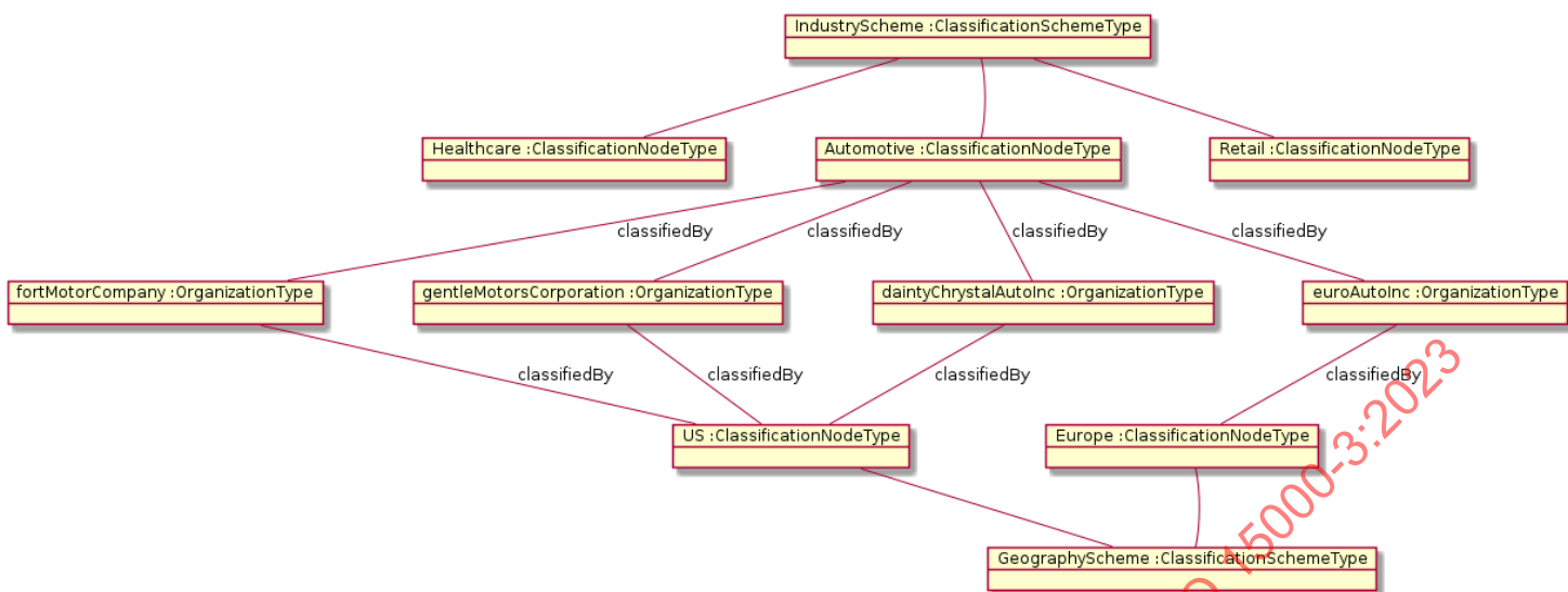
Figure 4 Classification example
