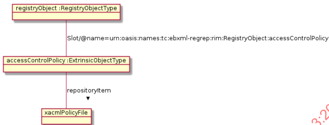
Figure 11 Assigning access control policy to a registry object
