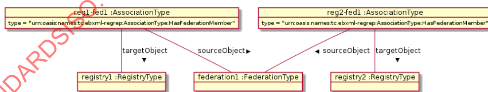
Figure 10 Federation information model
