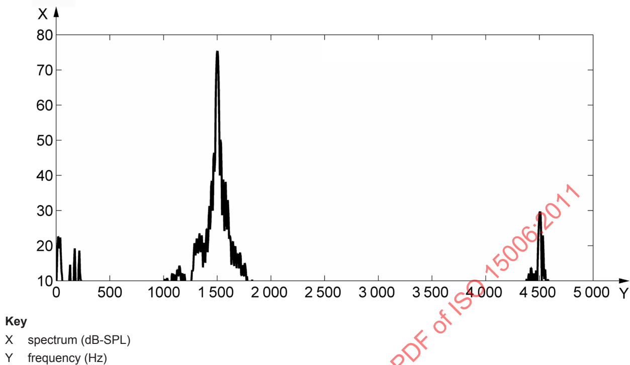
Figure A.1 — Spectrum for IVBSS FCW chime
