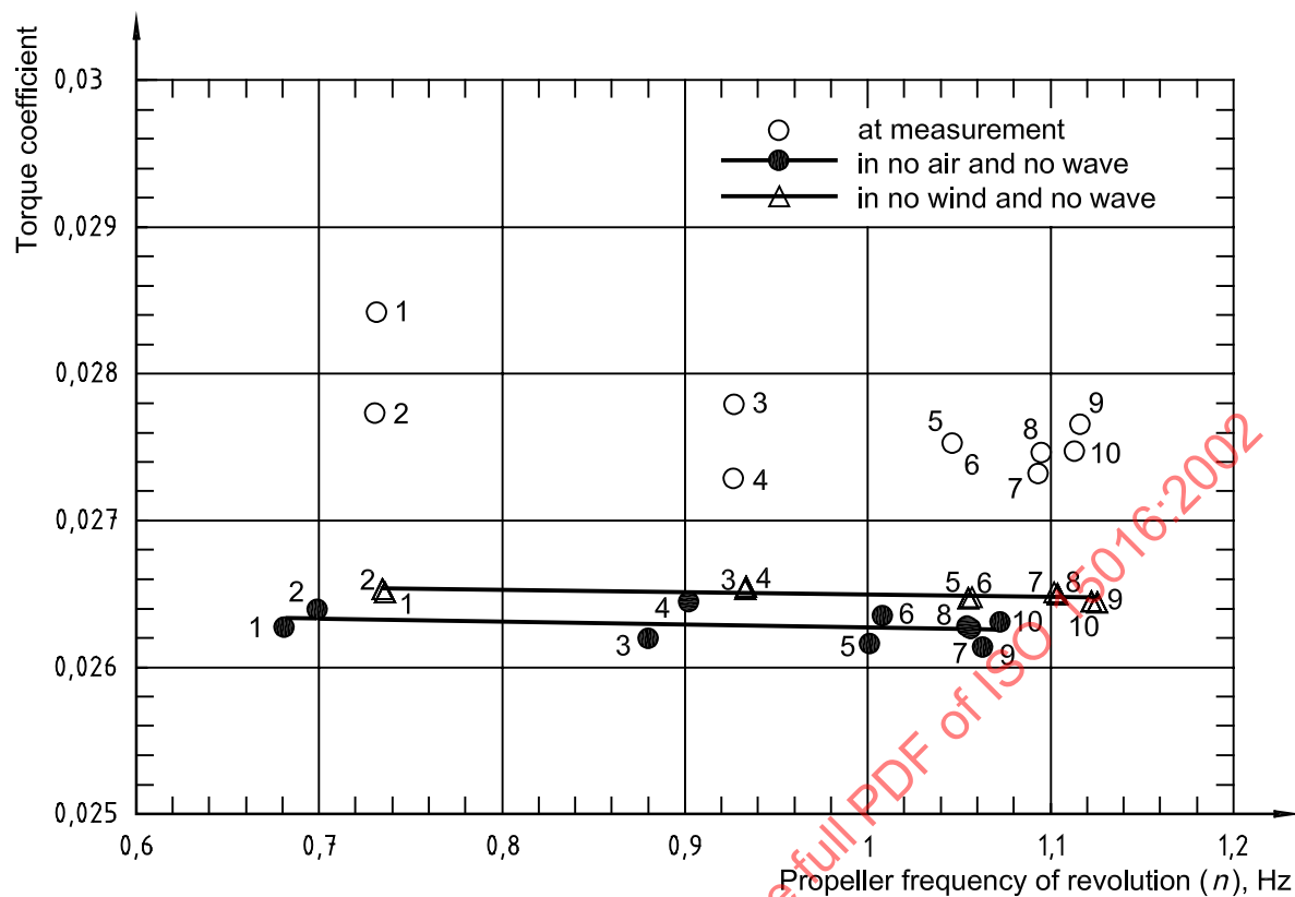
Figure 6 — Example of torque coefficient curves and propeller frequency of revolution
