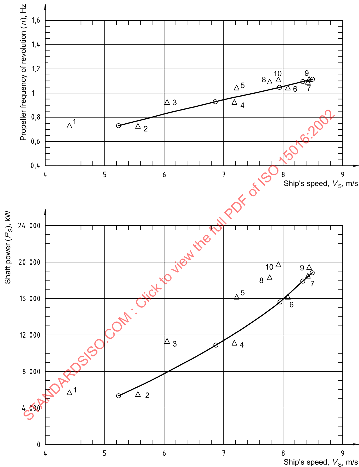
Figure 5 — Examples of trial performance curves
