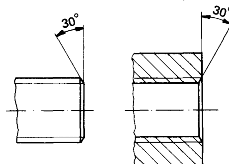
FIGURE 12 — Chamfer of start of thread
