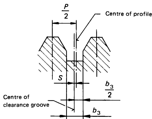
FIGURE 9 — Displacement of the clearance groove for the profile with truncated flanks
