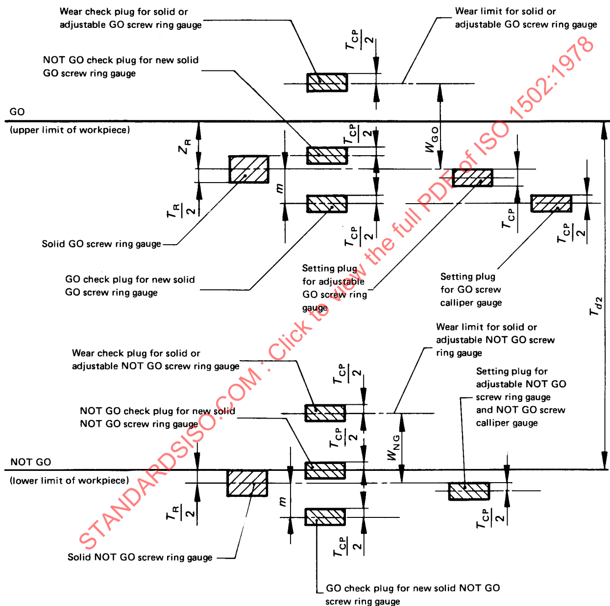
FIGURE 1 — Tolerance zones for the pitch diameter of gauges for external threads (diagram)
