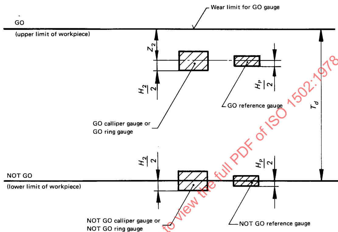
FIGURE 3 — Tolerance zones for plain gauges for major diameter of external threads (diagram)
