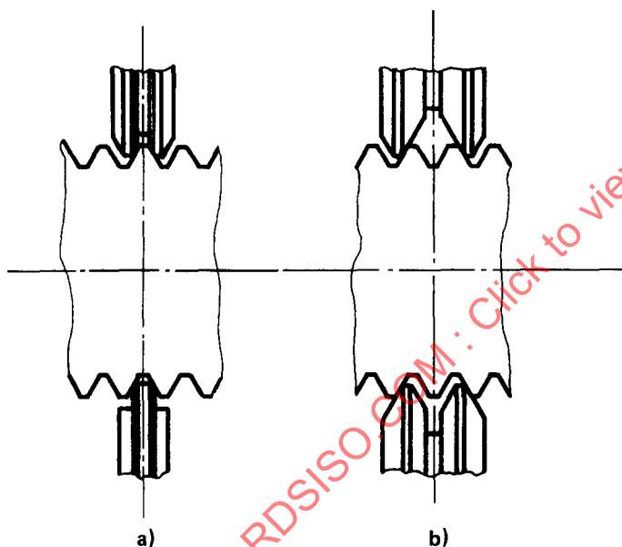
FIGURE 10 — NOT GO screw calliper gauge
