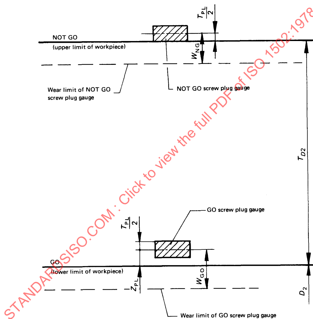
FIGURE 2 – Tolerance zones for the pitch diameter of gauges for internal threads (diagram)
