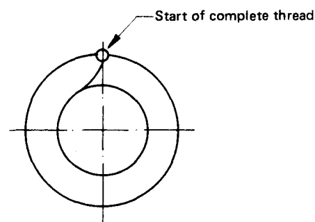
FIGURE 11 — Start of complete thread
