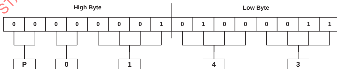
Figure 19 — Diagnostic trouble code encoding example DTC P0143
