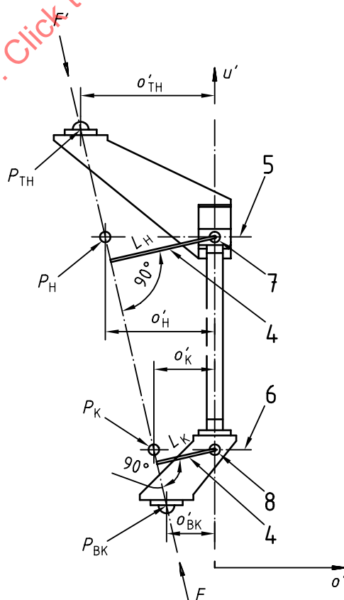
Figure 2 — Test configurations for A-P and M-L tests in f' - u' - and o' - u' - plane
