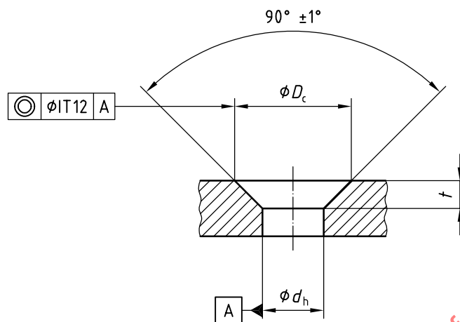
Figure 1 — Dimensions
