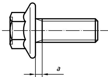
Figure 4 — Hexagon bolt with flange threaded to the head
