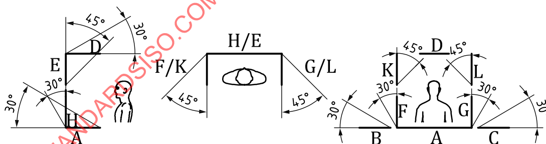
Figure A.2 — Recommended maximum angles for panels
