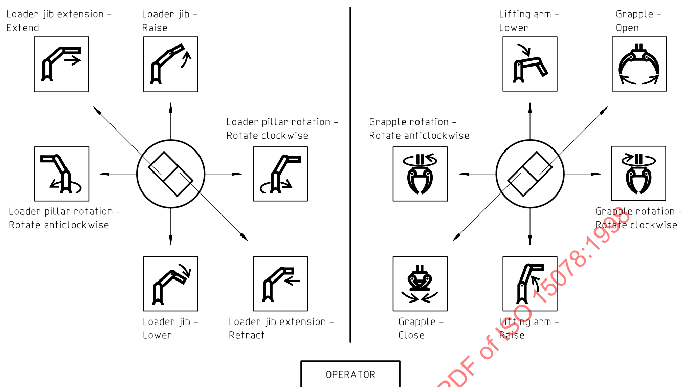
Figure 1 — Log loader controls, two-lever system operational pattern — System A
