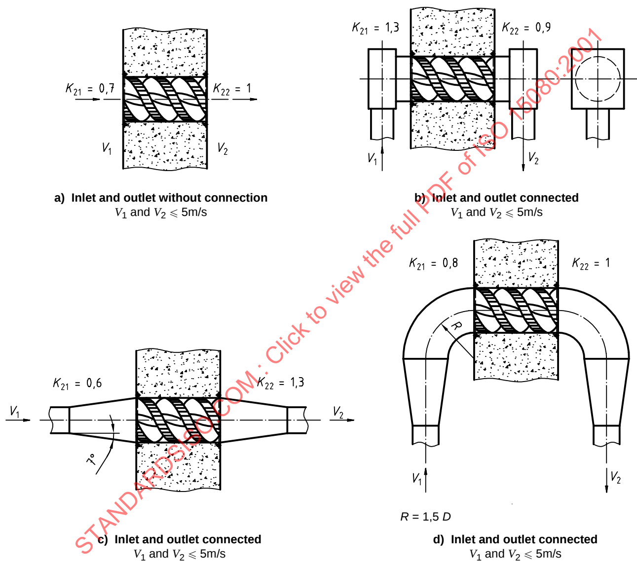
Figure A.2 — Diagram for calculation of coefficients of pressure drop K_{21} + K_{22}
