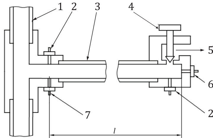
b) Example of transducer locations and bleed valve mounting
