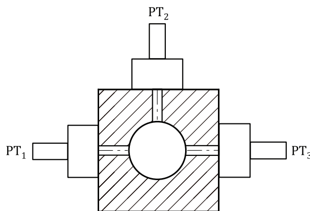
Figure 3 — Example of pressure transducer calibration distribution
