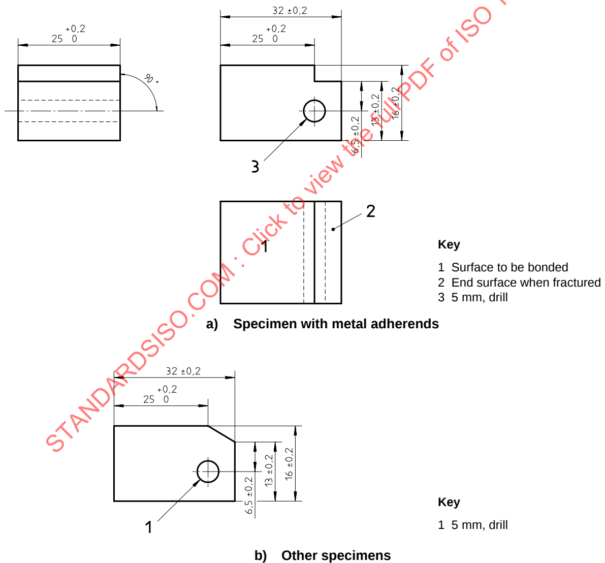
Figure 2 — Specimen shape and dimensions
