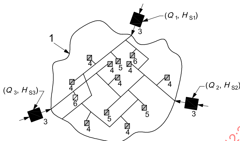
Figure 10 — Determination of a weighted-average calorific value (example)
