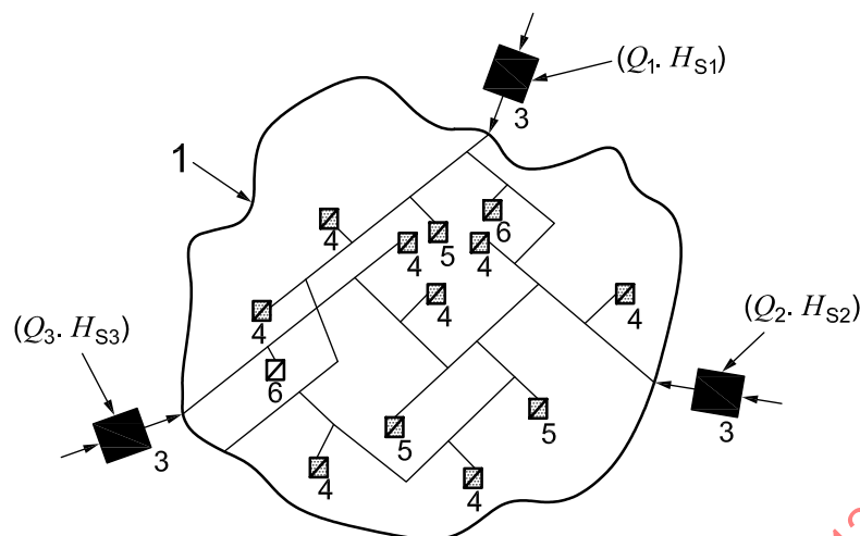
Figure 10 — Determination of a weighted-average calorific value (example)
