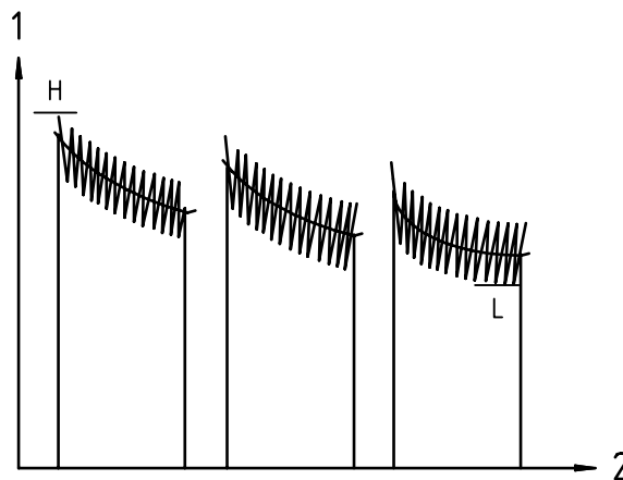
Figure 2 — Typical drift of results in extended tests
