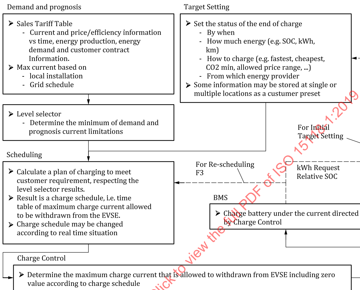
Figure A.6 — Example of charging only process flow chart
