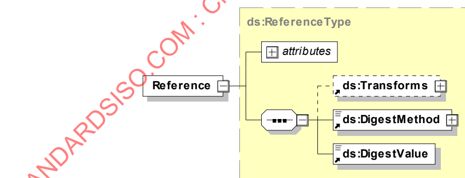
Figure 13 — Schema Diagram – Element Reference included in element SignedInfo
