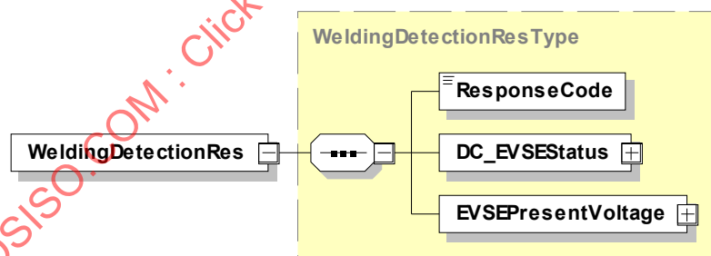
Figure 56 — Schema Diagram – WeldingDetectionRes
