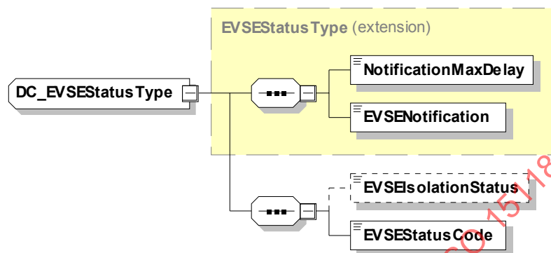
Figure 90 — Schema Diagram – DC_EVSEStatusType
