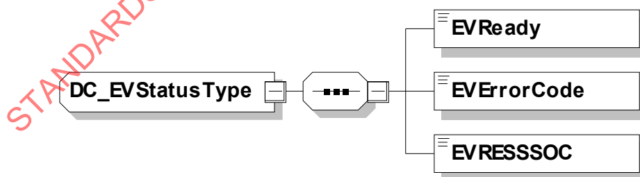
Figure 91 — Schema Diagram – DC_EVStatusType
