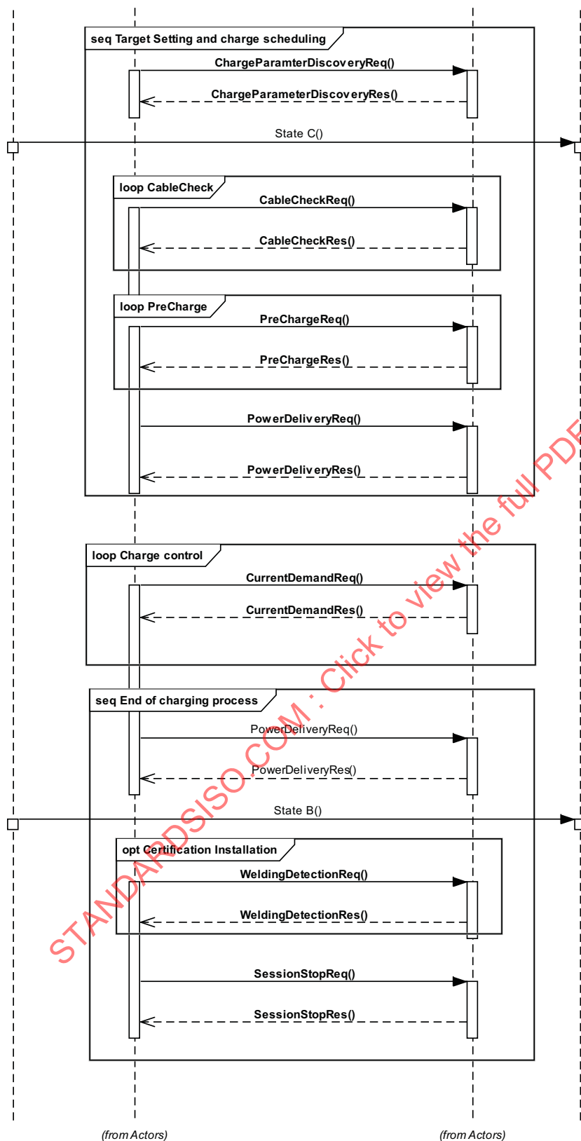
Figure 108 — Overview DC Request-Response Message Sequence PnC Identification Mode (2 of 2)
