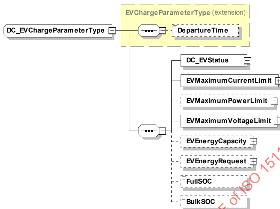
Figure 92 — Schema Diagram – DC_EVChargeParameterType
