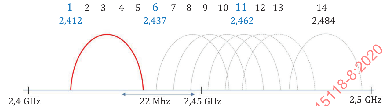
Figure B.2 — One WLAN Interferer is on channel 3 while channels 8 to 14 are interference free
