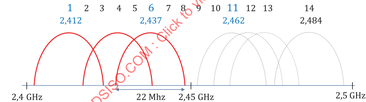
Figure B.3 — WLAN Interferers exist on channel 1, 4 and 6 while channels 11 to 14 are interference free
