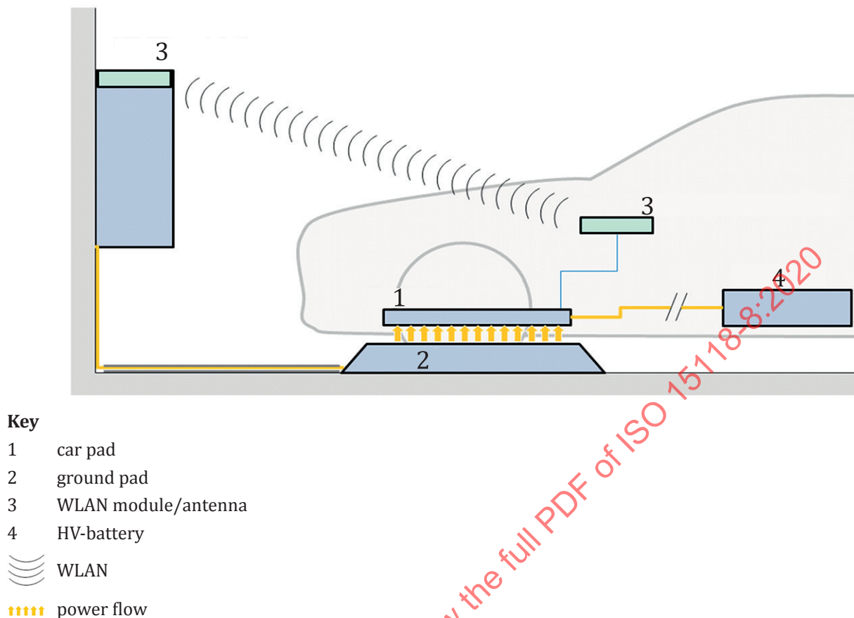
Figure A.2 — Typical distance between wireless communication modules/antennae in case of WPT
