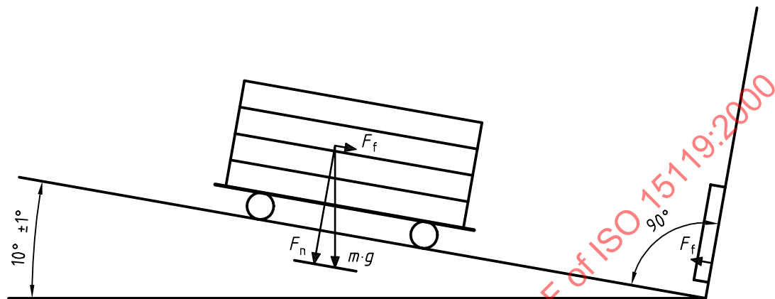
Figure 1 — Inclined plane method
