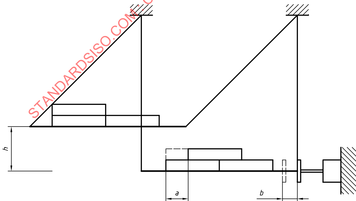
Figure 2 — Pendulum method
