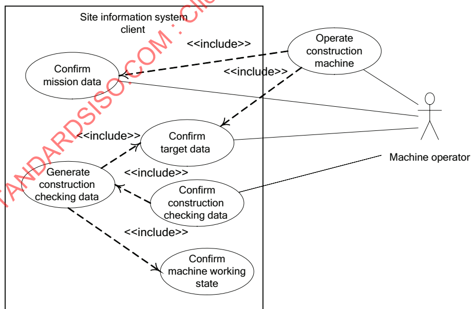
Figure D.5 — Use-case diagram — As-build judging service
