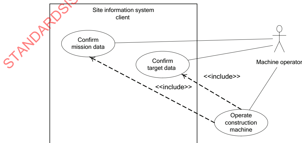
Figure D.4 — Use-case diagram — Machine operation supporting service
