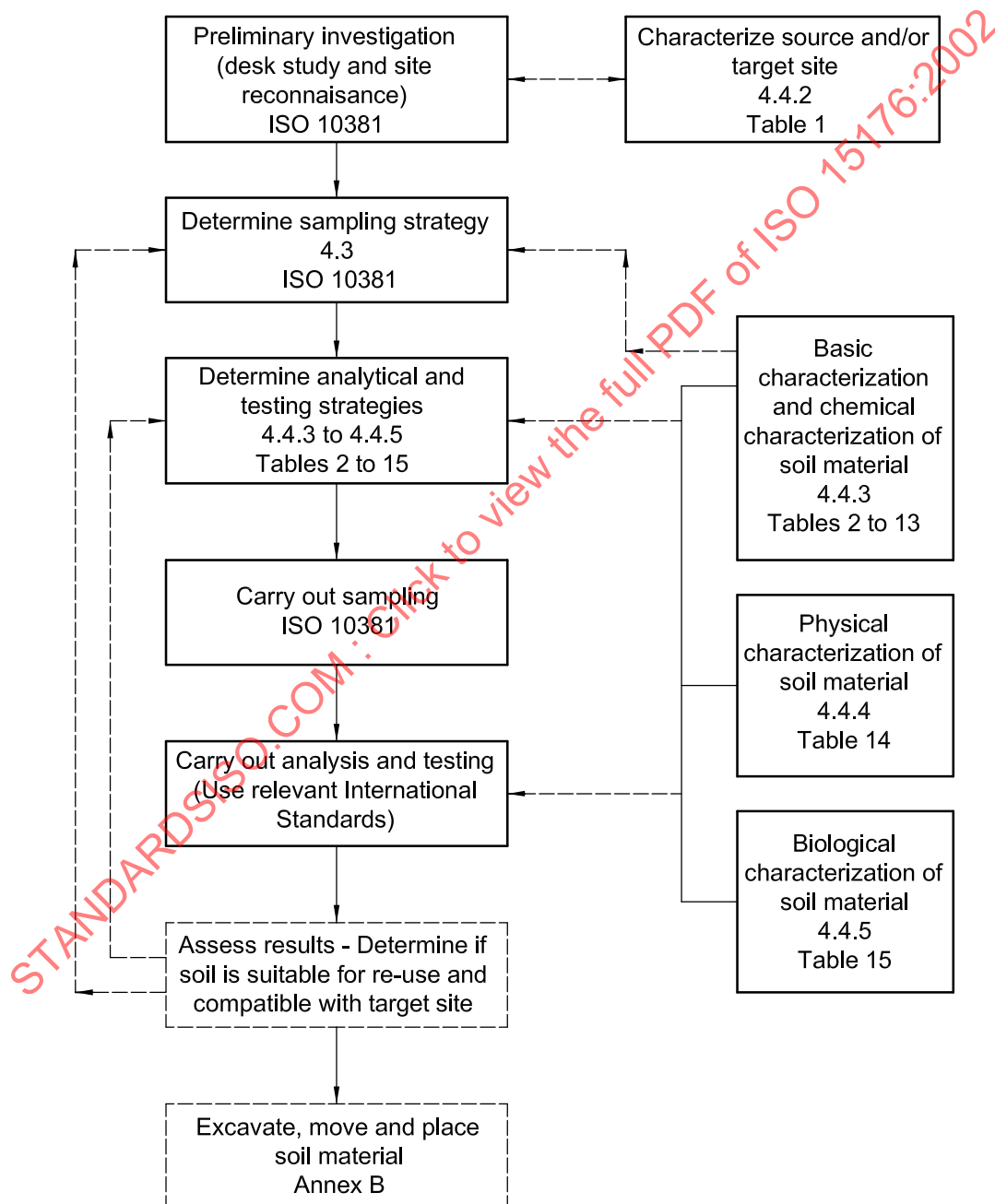
Figure 1 — Overall flow chart for characterization of soil materials for re-use
