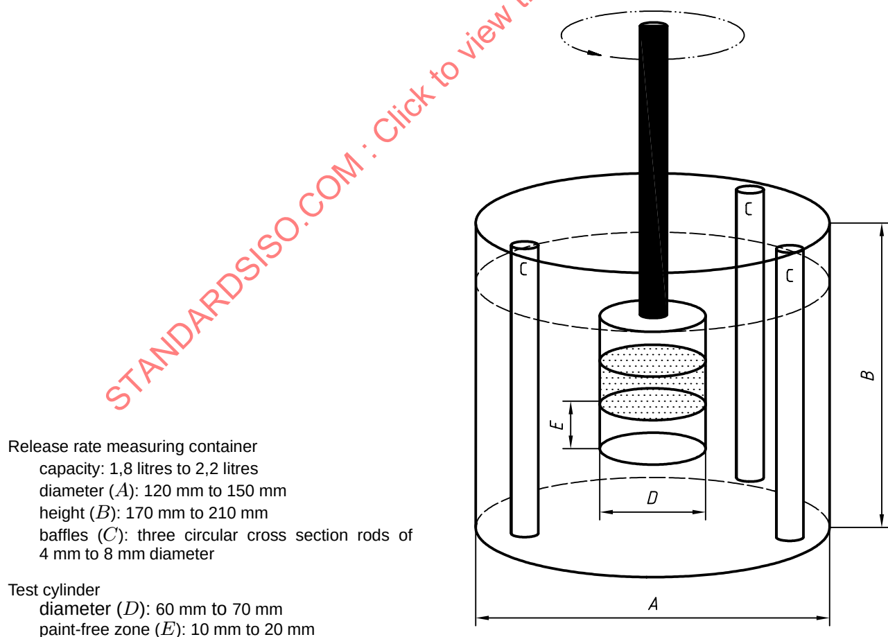
Figure 1 — Release rate measuring container
