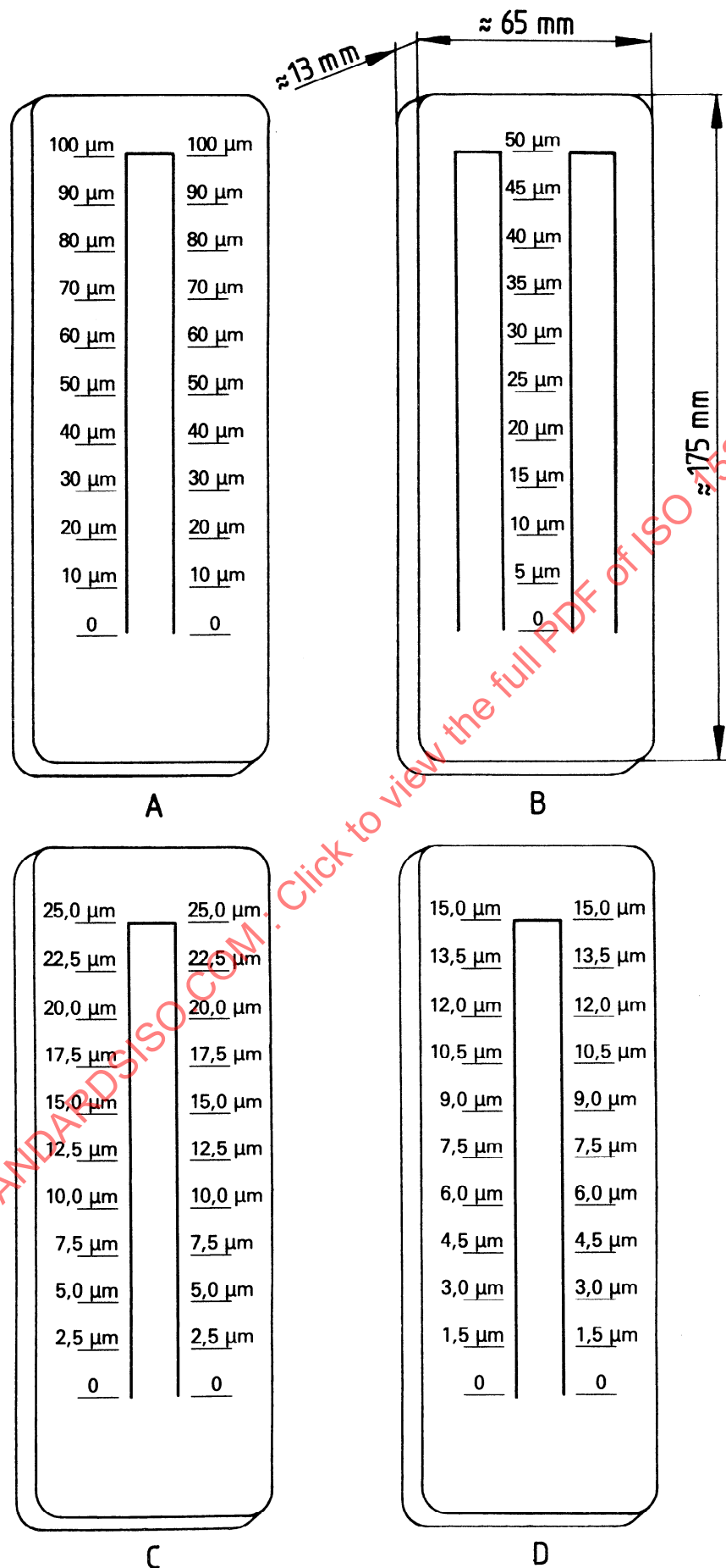
Figure 1 — Typical gauges
