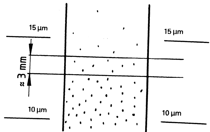
Figure 4 — Enlarged view of gauge reading 14 \mu\text{m}
