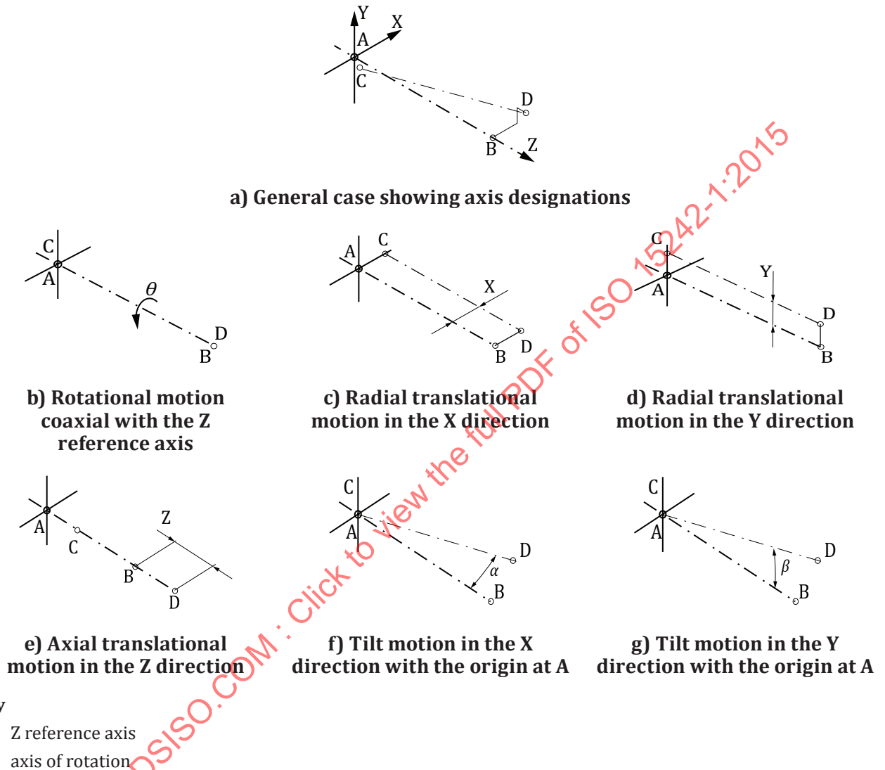
Figure 4 — Schematic diagrams of the six degrees of freedom of an axis of rotation
