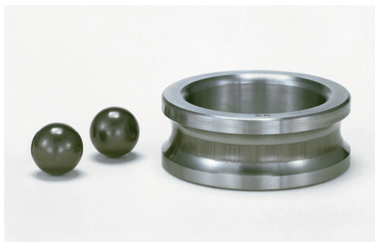
Figure 24 — Fluting on the inner ring raceway and matt dark grey coloured balls of a deep groove ball bearing
