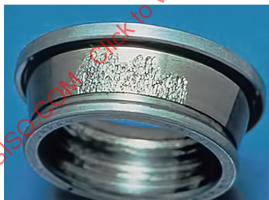
Figure 4 — Advanced subsurface spalling in a tapered roller bearing — Stationary inner ring
