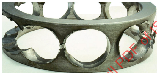
Figure 9 — Advanced abrasive wear on the cage pockets of a solid metal cage
