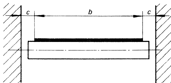
FIGURE 2 — Return idler
