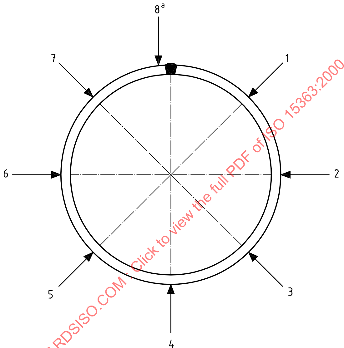
Figure 3 — Wall thickness measurement positions
