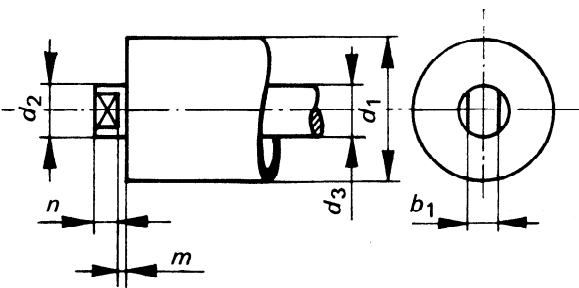
FIGURE 5 — Spindle end without added end cap
