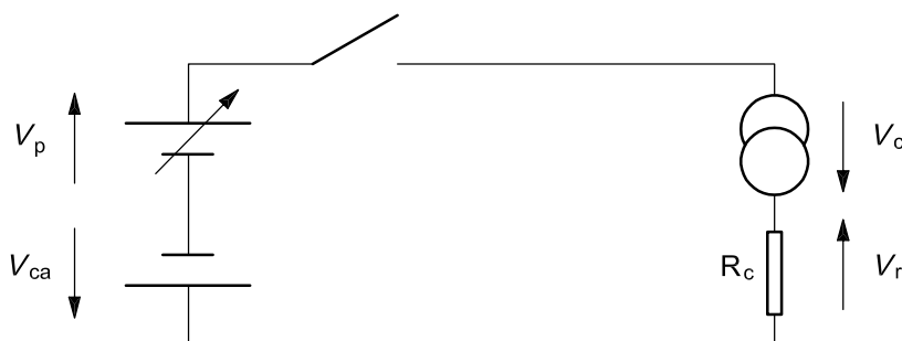
Figure 7 — Electrical diagram
