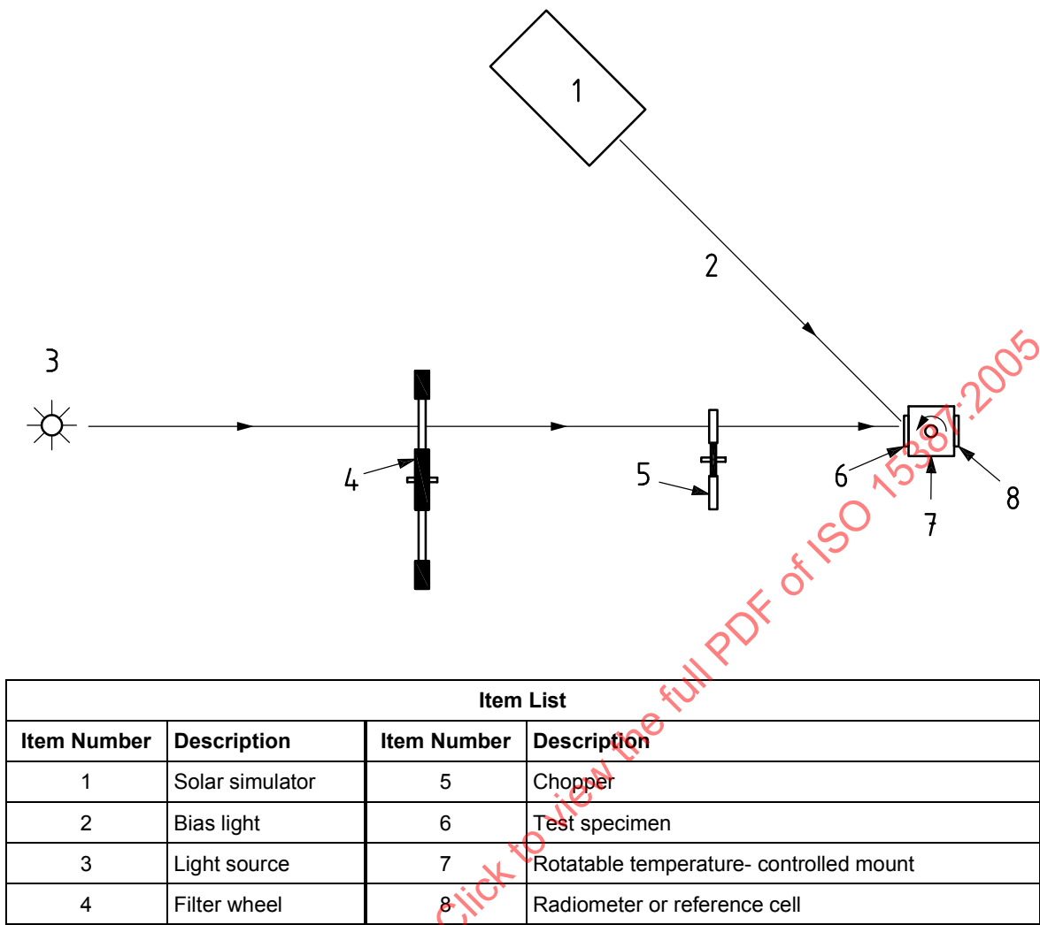
Figure C.2 — Spectral response measurement using a filter wheel
