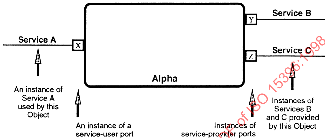
Figure 1-1b: Drawing Conventions for an Object-Instance
