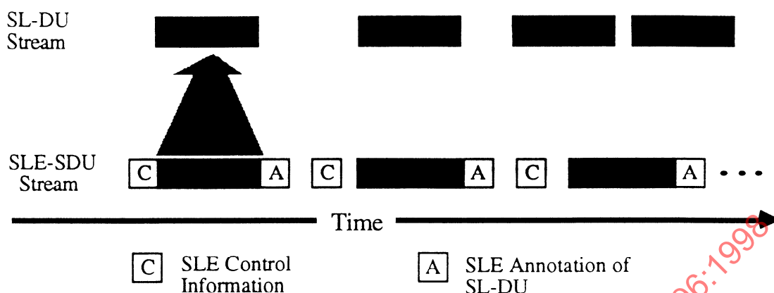
Figure 3-4b: An illustration of Mapping Forward SLE-SDUs to Forward SL-DUs
