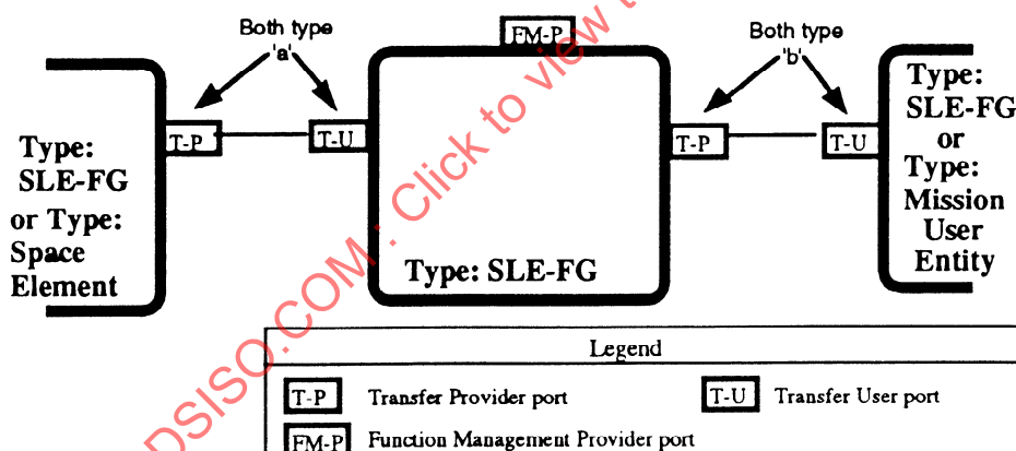
Figure 4-3: Interconnection of SLE-FGs Ports
