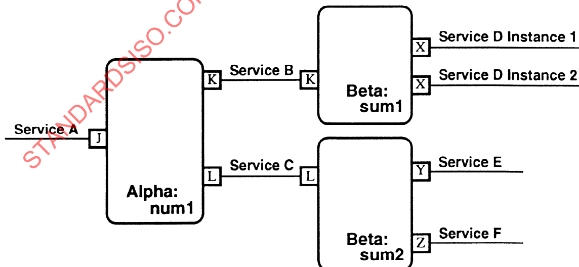
Figure 1-1c: Drawing Conventions for Multiple Object-Instances
