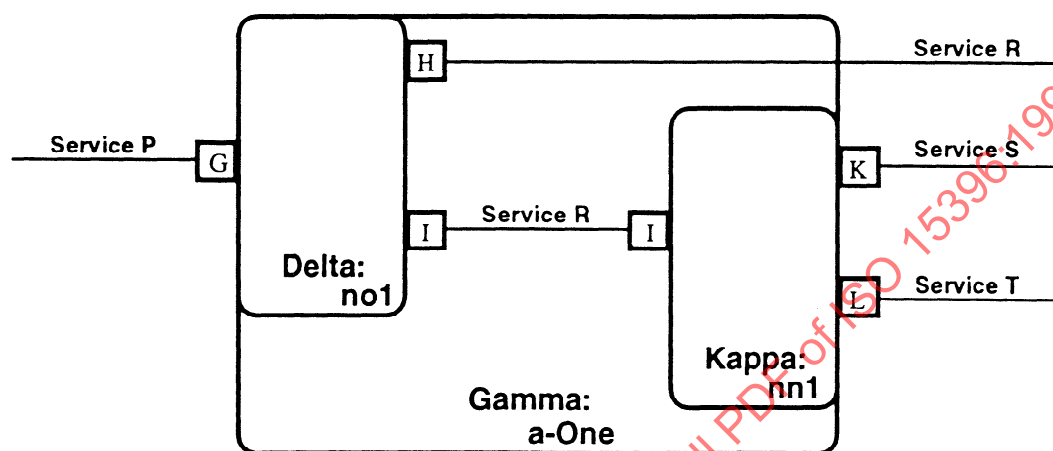
Figure 1-2: Object Refinement
