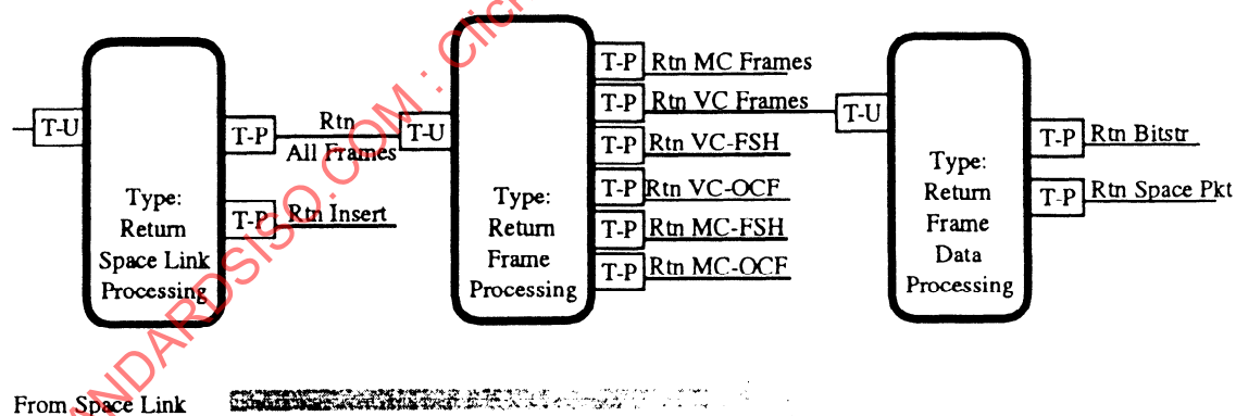
Figure 4-4: Return Functional Groups
