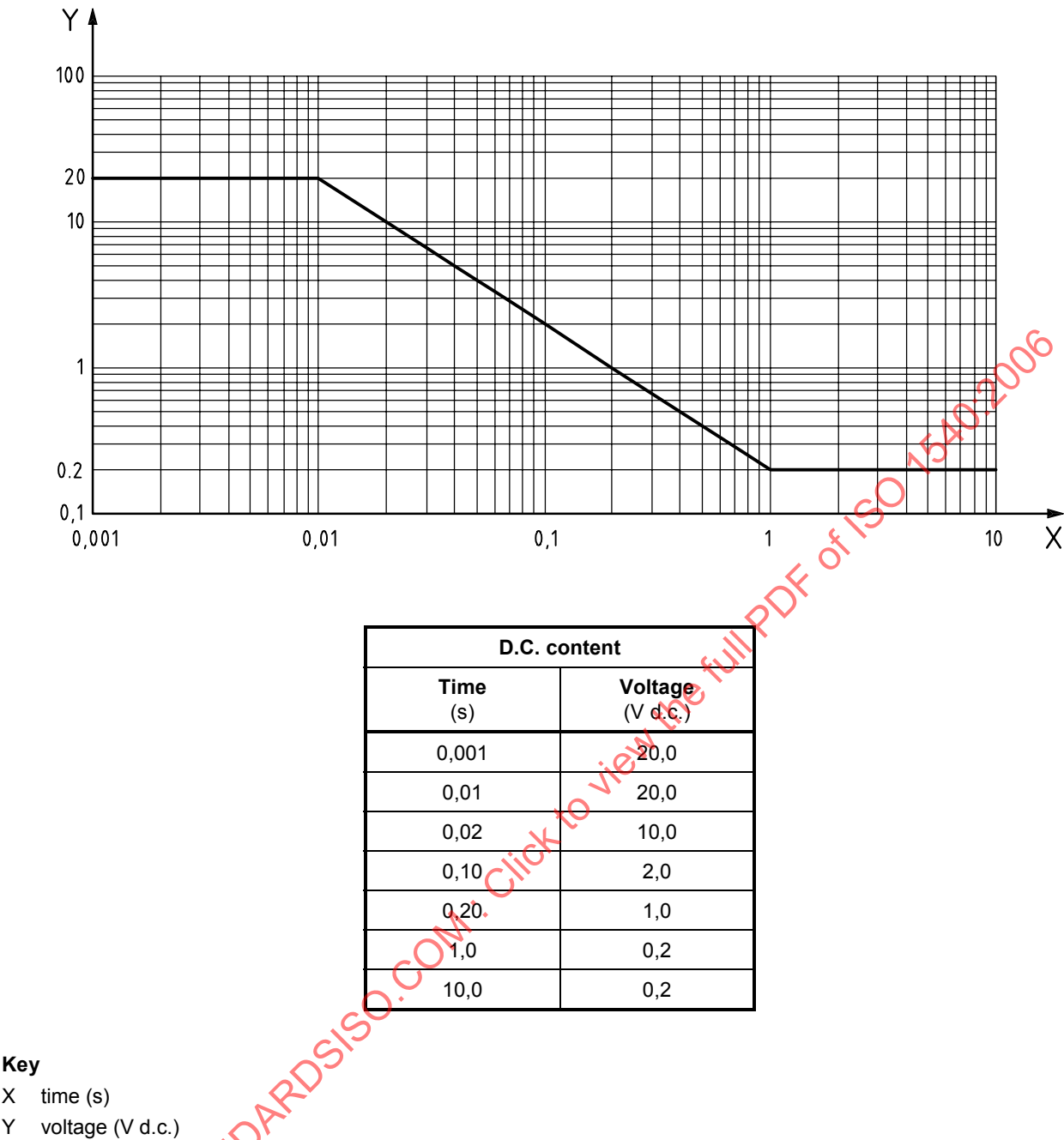
Figure 10 — Abnormal d.c. content transient on a.c. input power (constant frequency and variable frequency)
