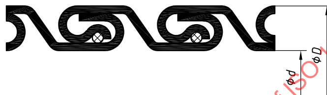
Figure 4 — Cross-section of a type DOP, double overlap, packed hose
