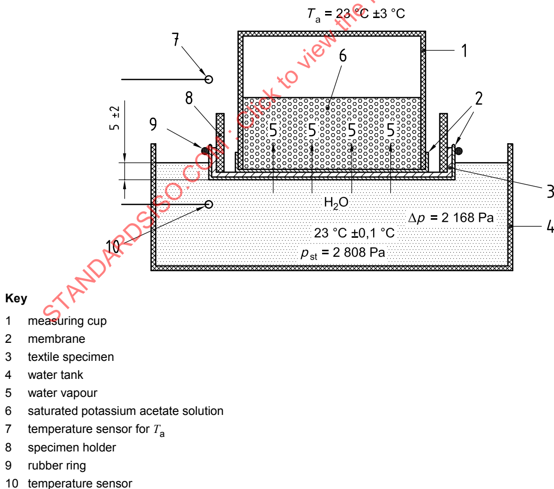
Figure 1 — Schematic test arrangement for the cup method
