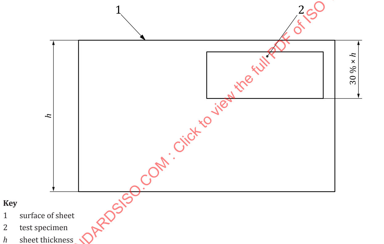
Figure 3 — Taking test specimens from sheets of thickness > 20 mm but < 200 mm
