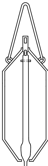
Figure 7 — Bottom or zone sampler (sectional view)
