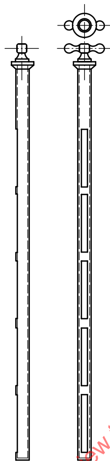
Figure 3 — Sampling tube consisting of two concentric tubes
