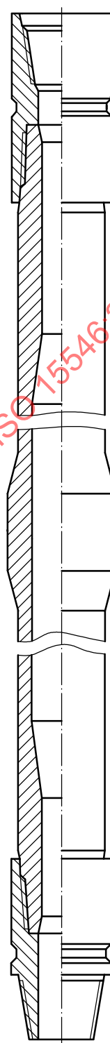
Figure 3 — Drill pipe with protector thickening
