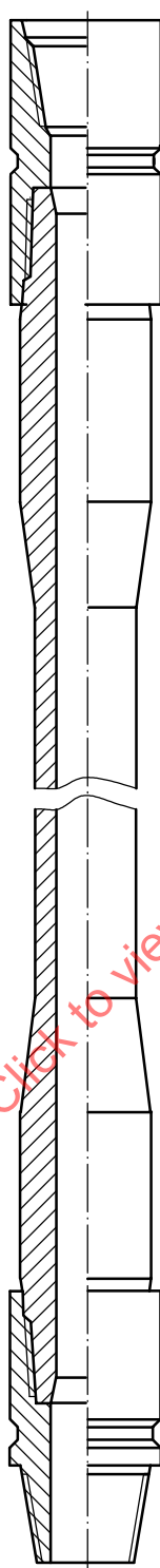
Figure 2 — Drill pipe with external upset
