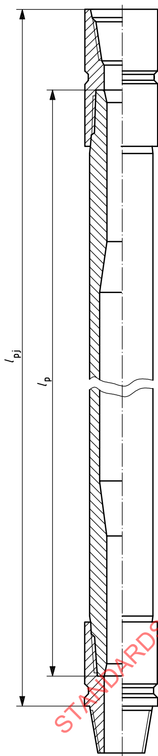
Figure 1 — Drill pipe with internal upset
