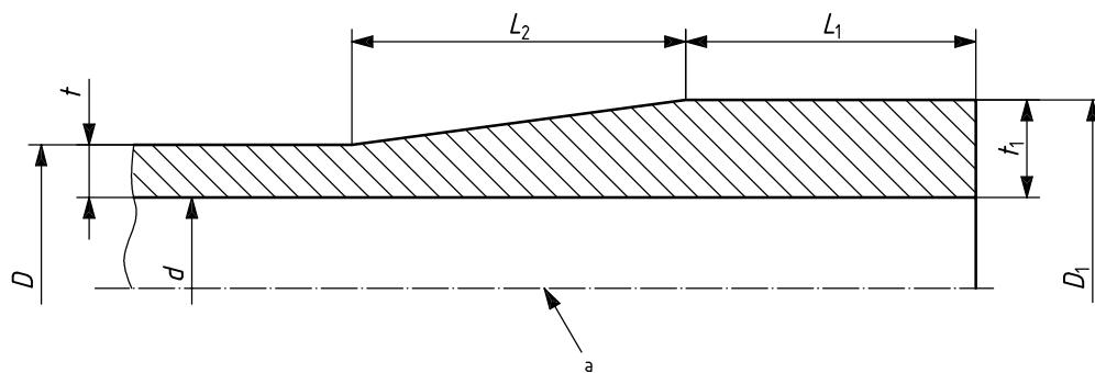
Figure 4 — Drill pipe end with external upset
