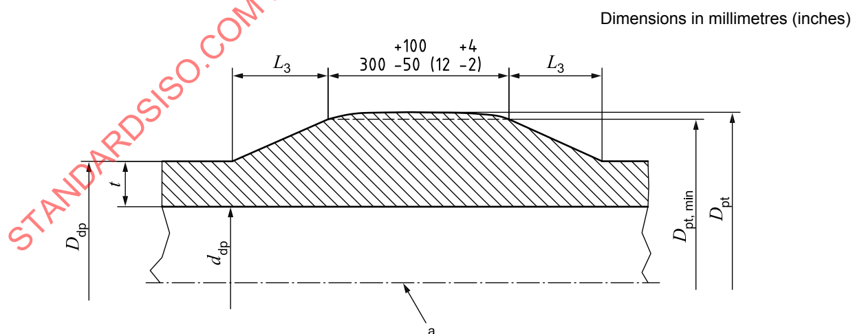
Figure 6 — Aluminium alloy drill pipe body end with internal upset (see Table 4)
