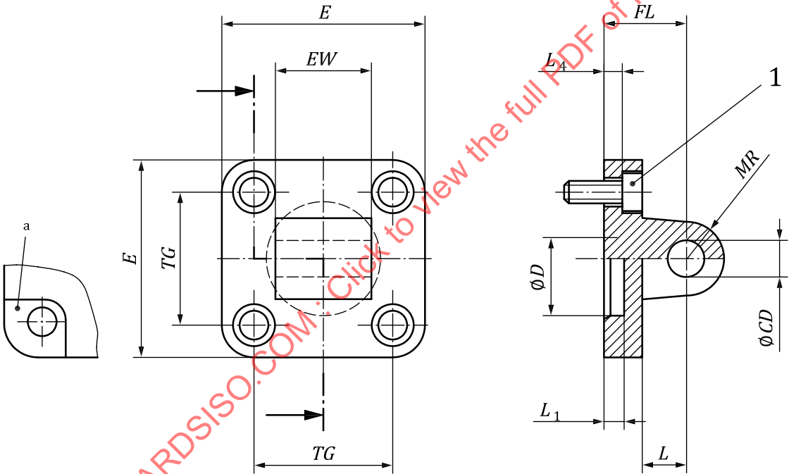
Key 1 cap screw a Optional open counterbore.
