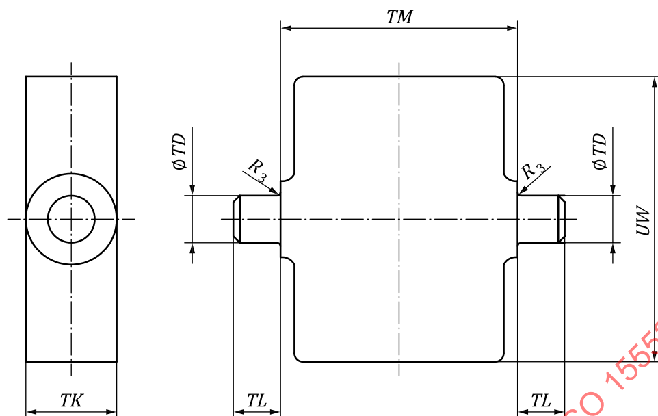
Figure 9 — Intermediate fixed or movable trunnions (male) (MT4)
