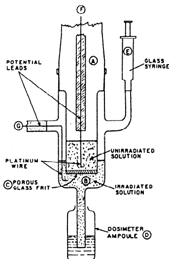
FIG. X1.1 Electrochemical Cell
