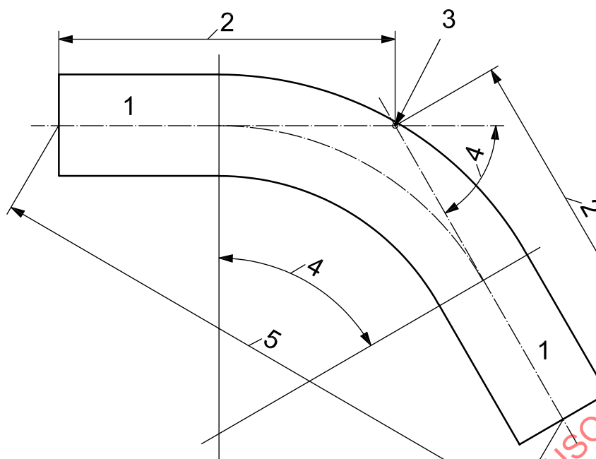
a) Bends with angles of 15^\circ and greater
