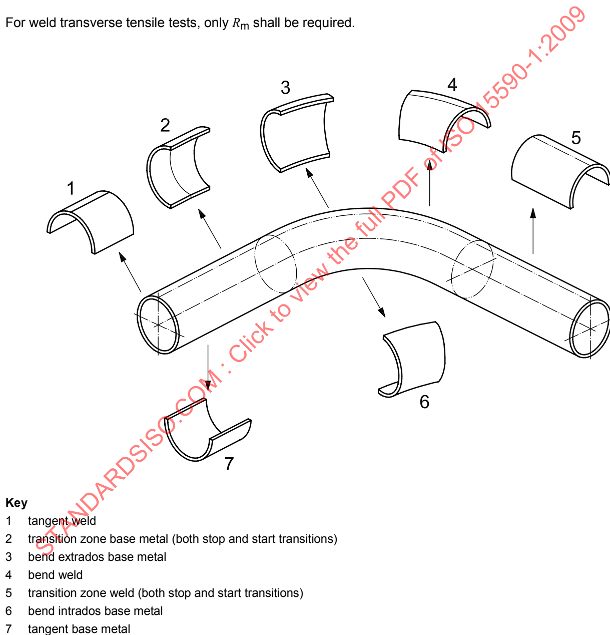
Figure 1 — Location for extraction of samples for testing
