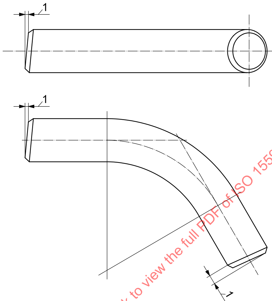
Figure 5 — Determination of end out-of-squareness
