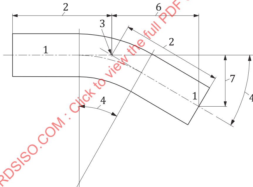
b) Bends with angles of less than 15°
