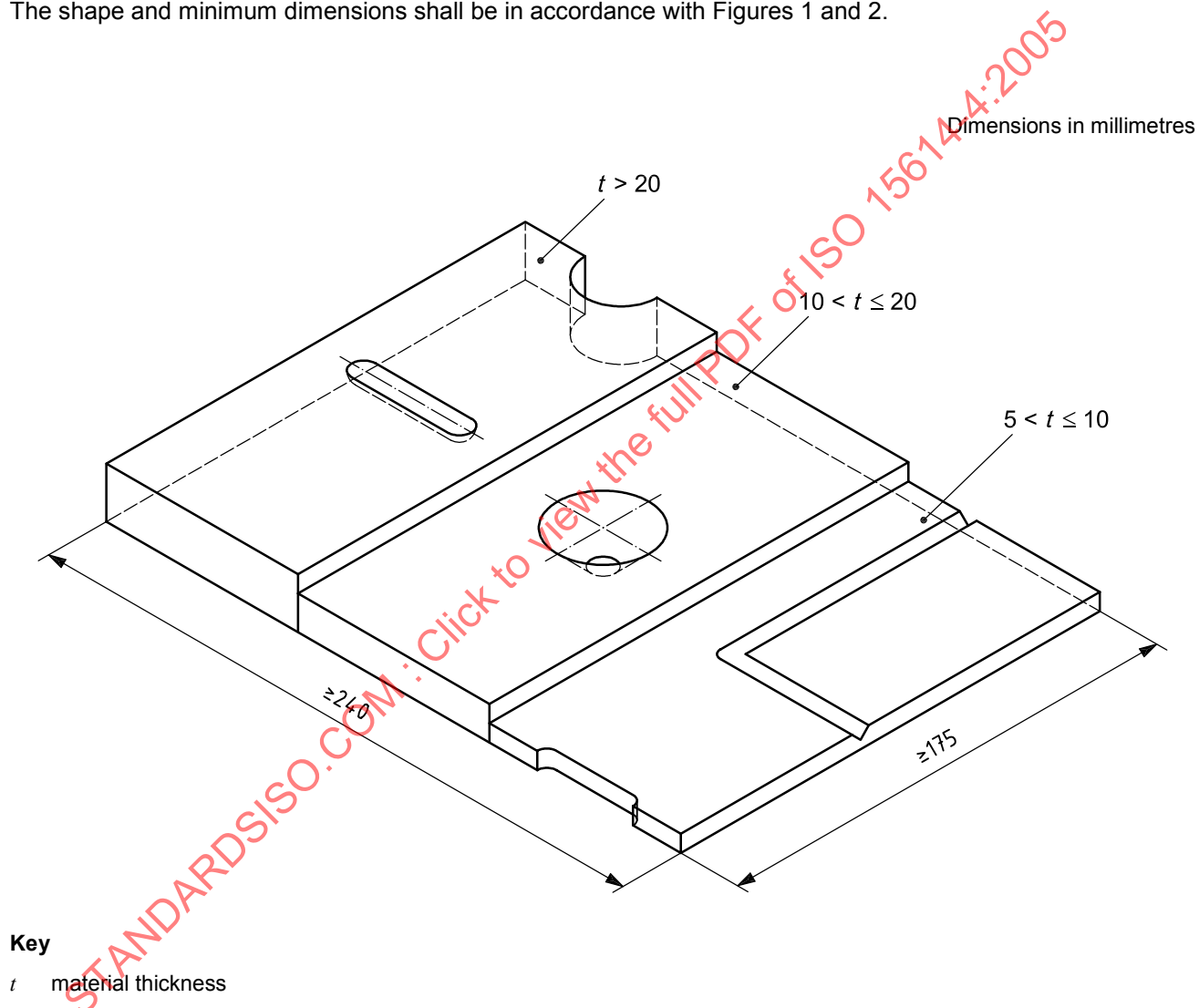
Figure 1 — Combined test piece with slot, hole and groove
