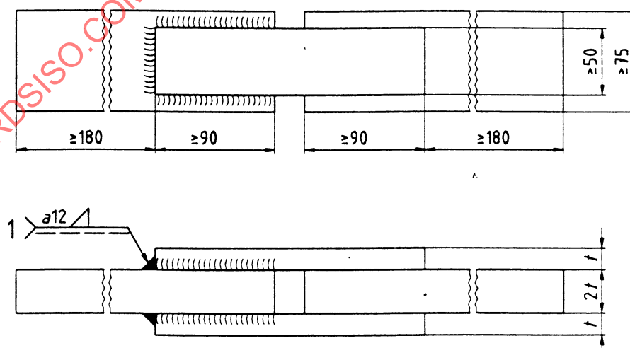
Figure 4 - Dimensions of test piece for fillet weld longitudinal from plate (lap joint)
