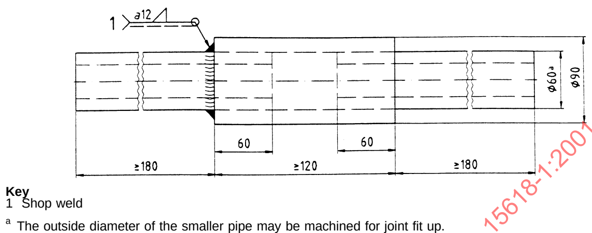
Figure 5 - Dimensions of test piece for fillet weld transverse from pipe (lap joint)
