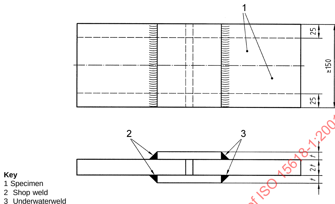
Figure 9 - Fillet weld shear strength specimen, transverse from plate
