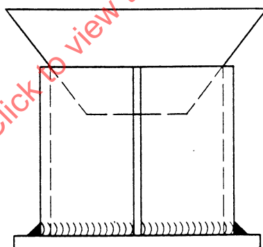
Figure 12 - Preparation and fracture testing of test specimens for a fillet weld on pipe
